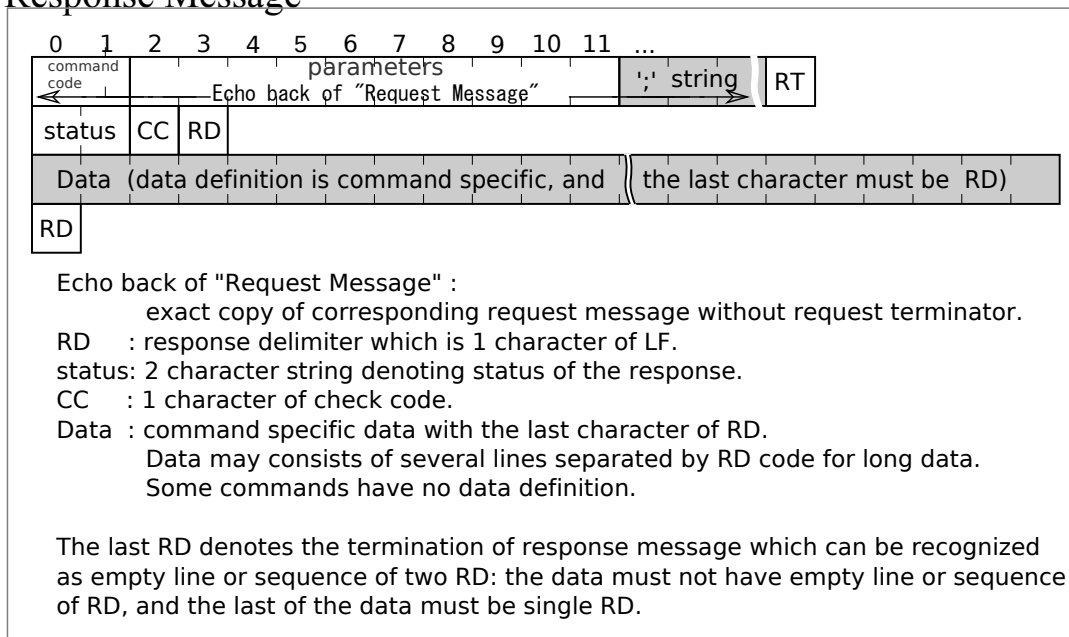
Figure 2.3: Response Message Format
