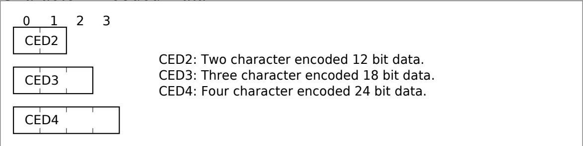
Figure 2.5: Character Encoded Format
