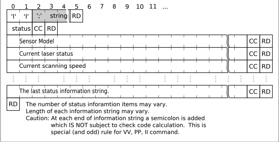
Figure 3.20: II Message Format
