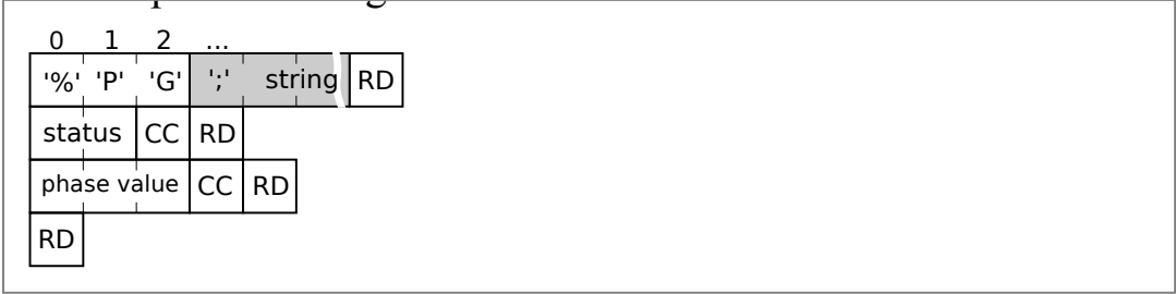
Figure 3.21: %PG Message Format
