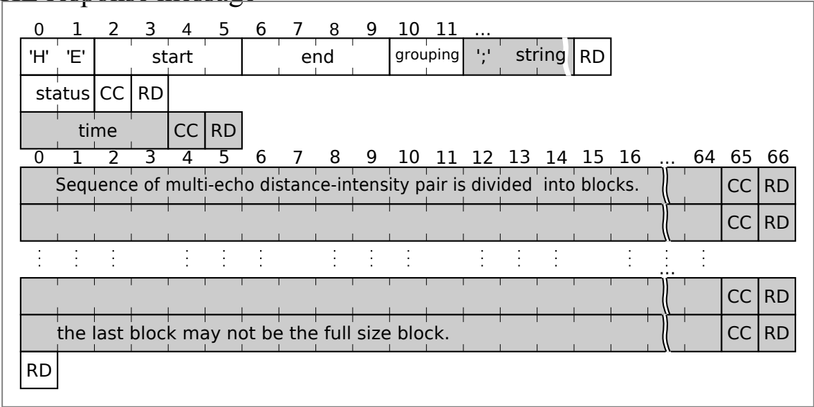
Figure 3.5 : HE Message Format
