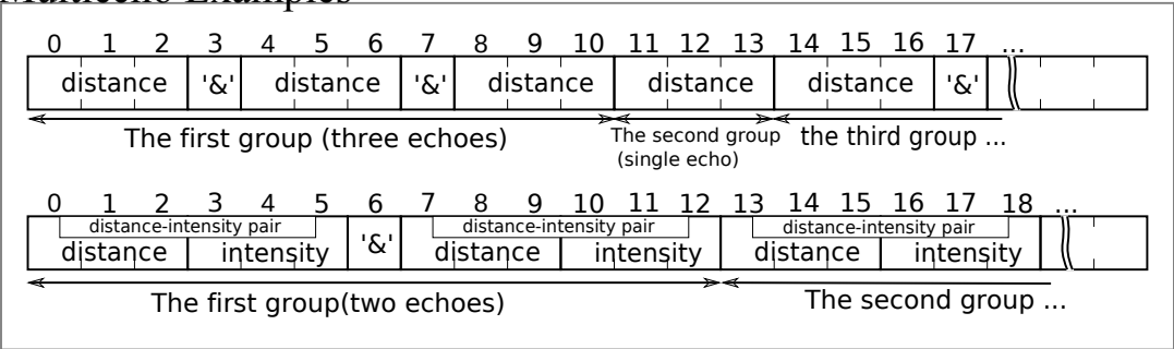
Figure 2.9: Multi- Echo Data Format
