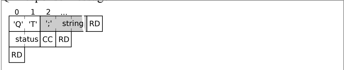
Figure 3.12: QT Message Format
