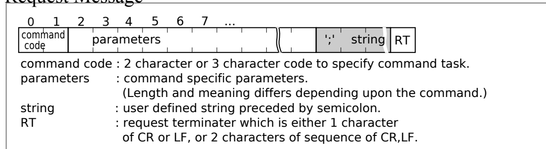
Figure 2.1: Request Message Format
