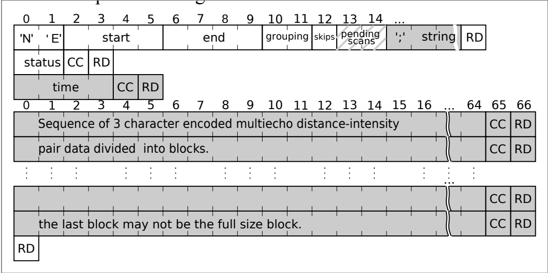
Figure 3.9 NE Message Format
