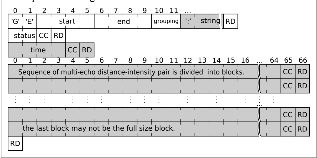
Figure 3.3 GE Message Format
