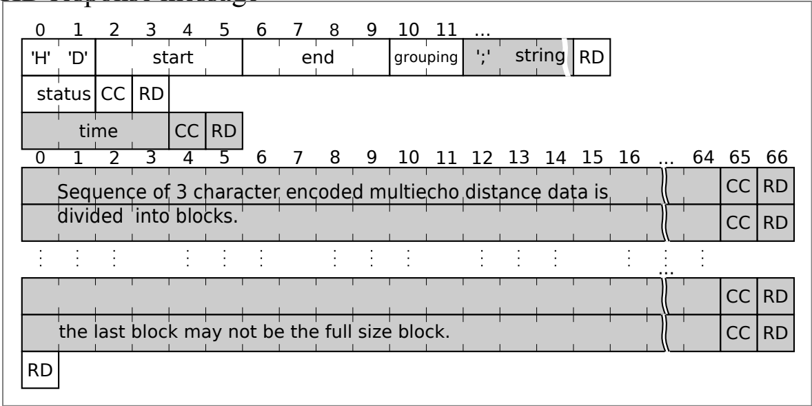
Figure 3.4: HD Message Format
