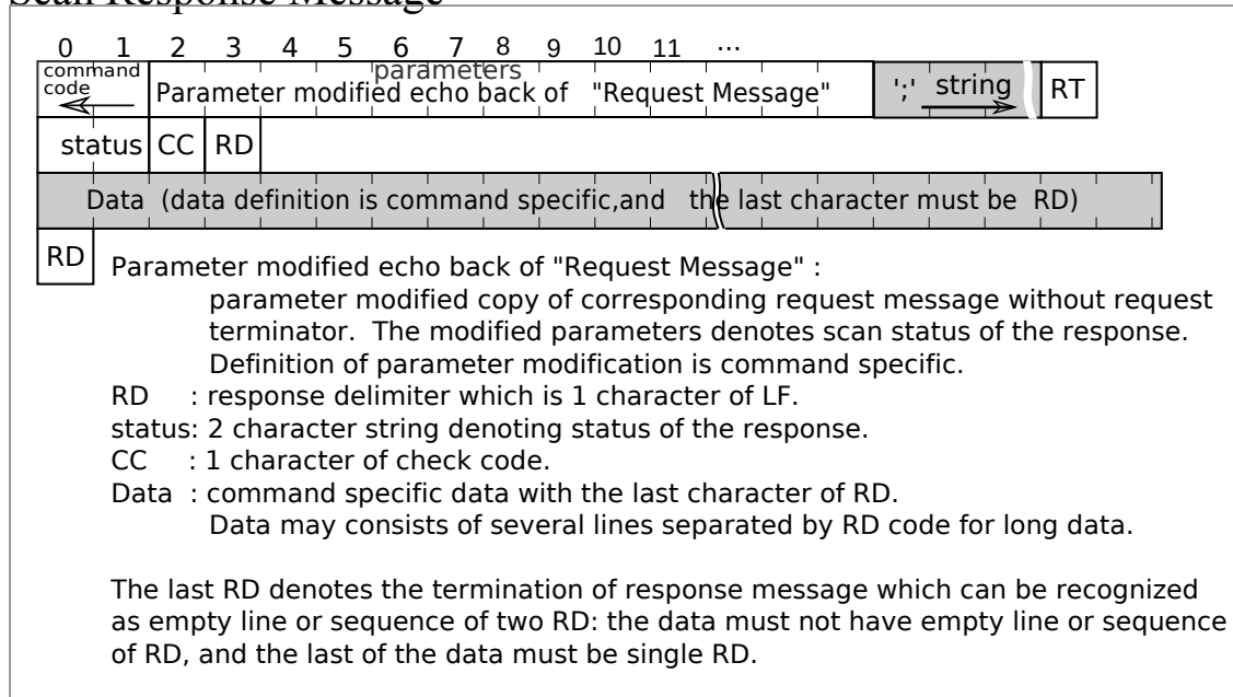
Figure 2.4 Scan Response Message Format
