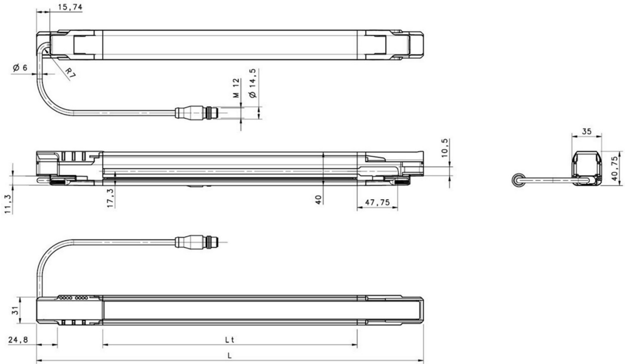
Fig 75 - Overall dimensions (mm)
