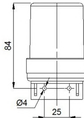
Fig 105 - Lamp LMS-2
