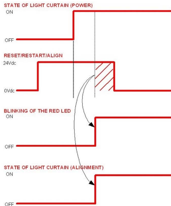
Fig 35 - Alignment timings
