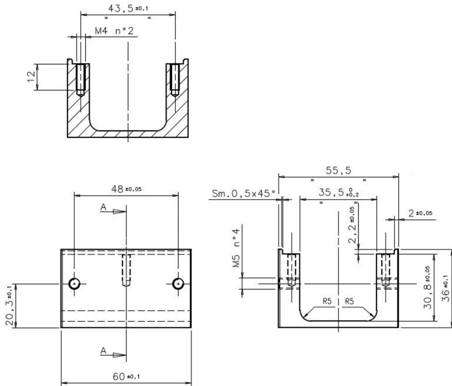
Fig 110 - Mounting bracket
