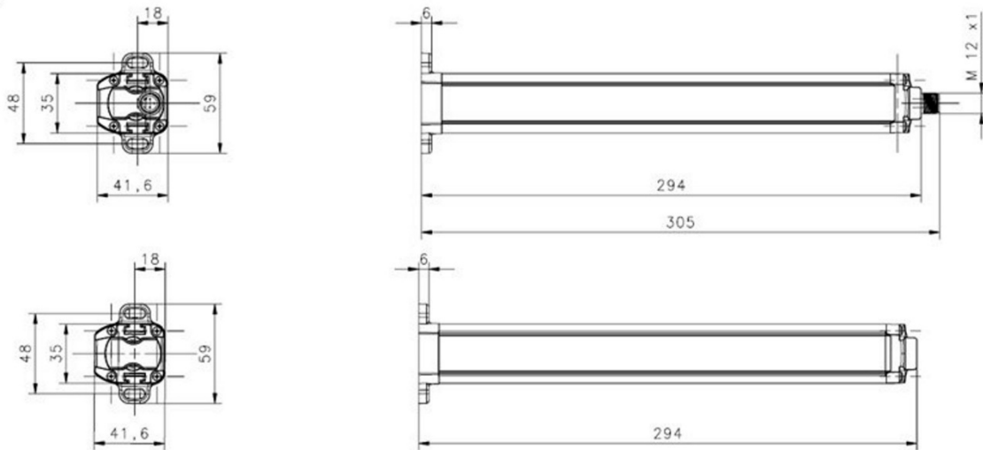
Fig 109 - Dimensions (mm)
