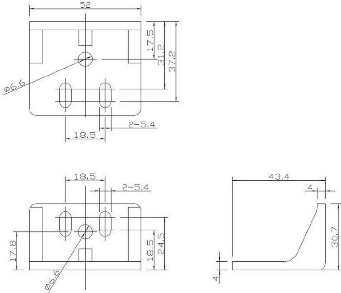
Fig 84 - ST-KPxMP
