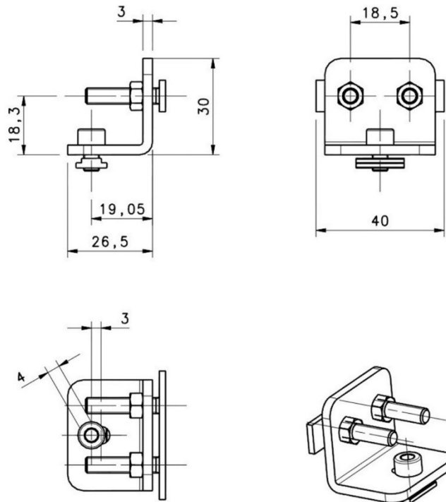
Fig 90 - Fixing kit
