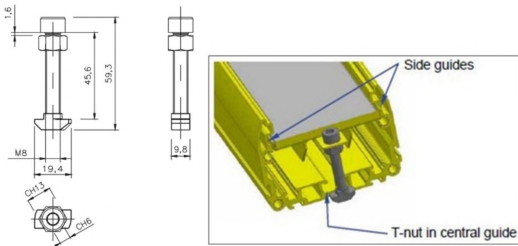
Fig 97 - Mounting kit
