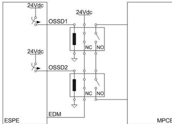
Fig 48 - PNP configuration
