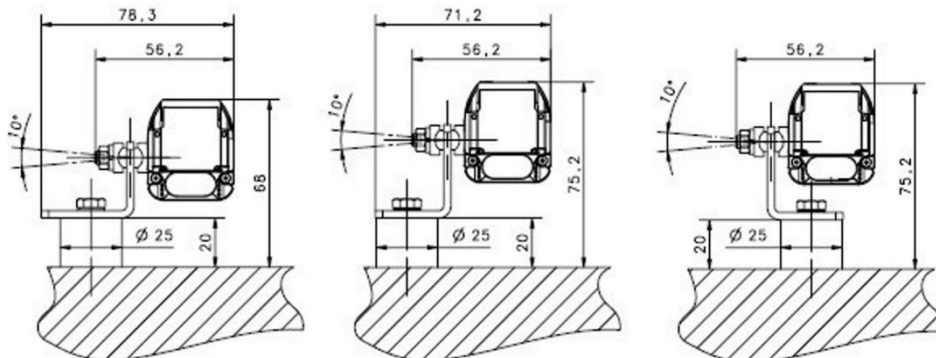
Fig 83 - Angled fixing bracket + Orientable support + Antivibration support
