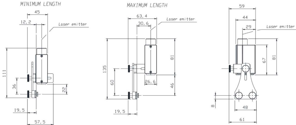
Fig 100 - Dimensions (mm)
