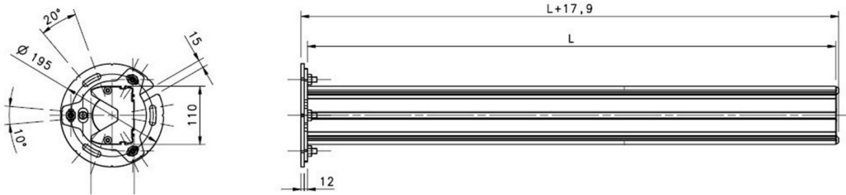
Fig 89 - Dimensions (mm)
