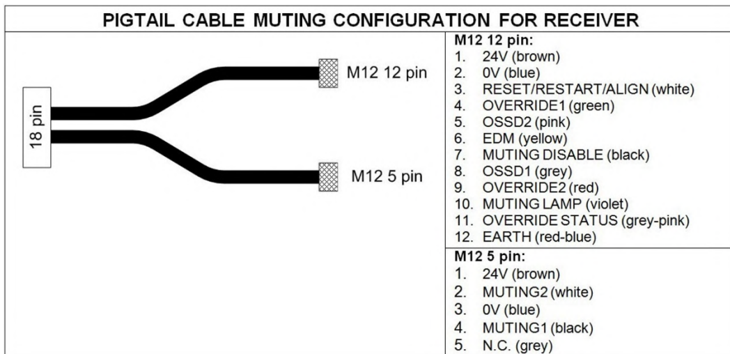
Fig 25 - Pigtail cable - Muting configuration for receiver RX (CS-R1-75-B-002)
