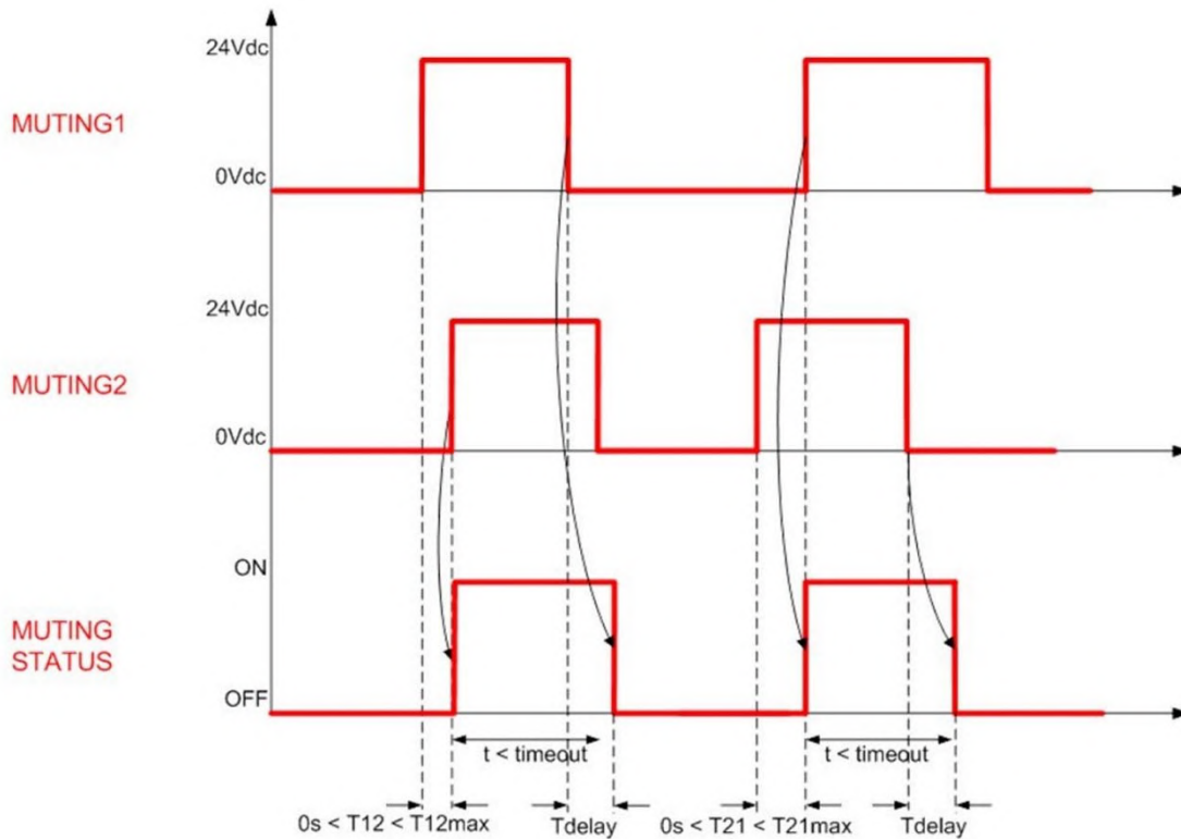
Fig 58 - T Muting timings
