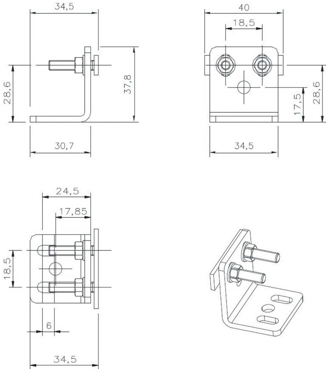
Fig 79 - ST-KSTD
