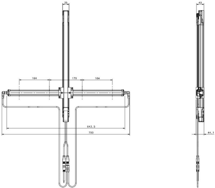
Fig 114 - Light curtain + Active/Passive arms T
