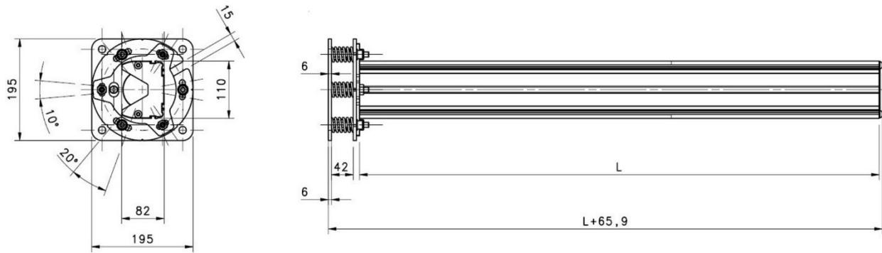
Fig 92 - Mounting
