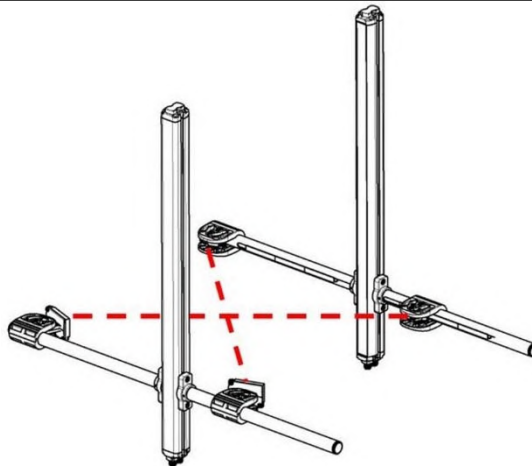
Fig 117 - X-MUTING
