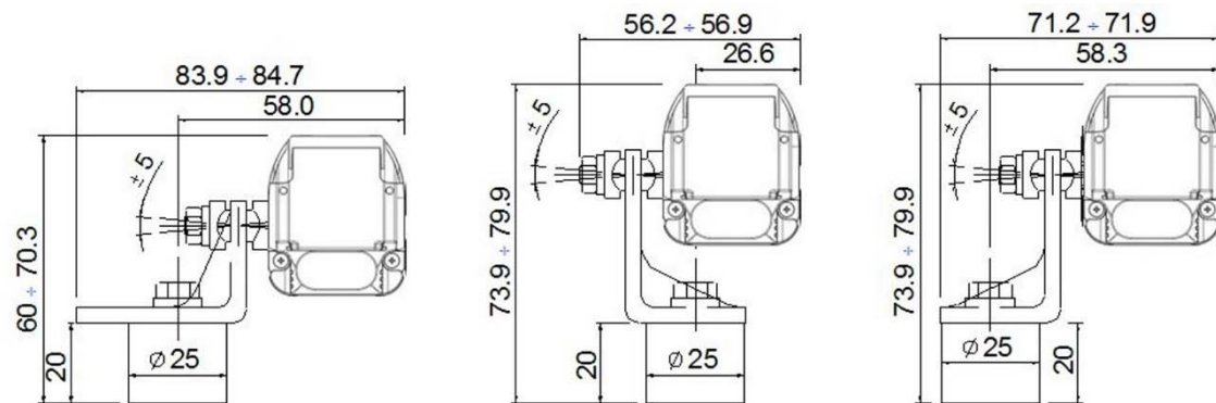
Fig 88 - Angled fixing bracket + Orientable support + Antivibration support
