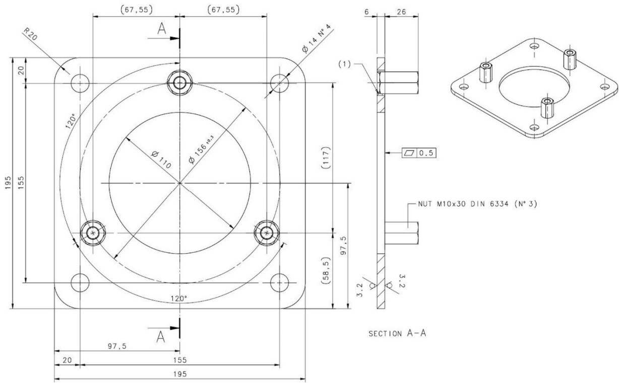
Fig 91 - Dimensions (mm)
