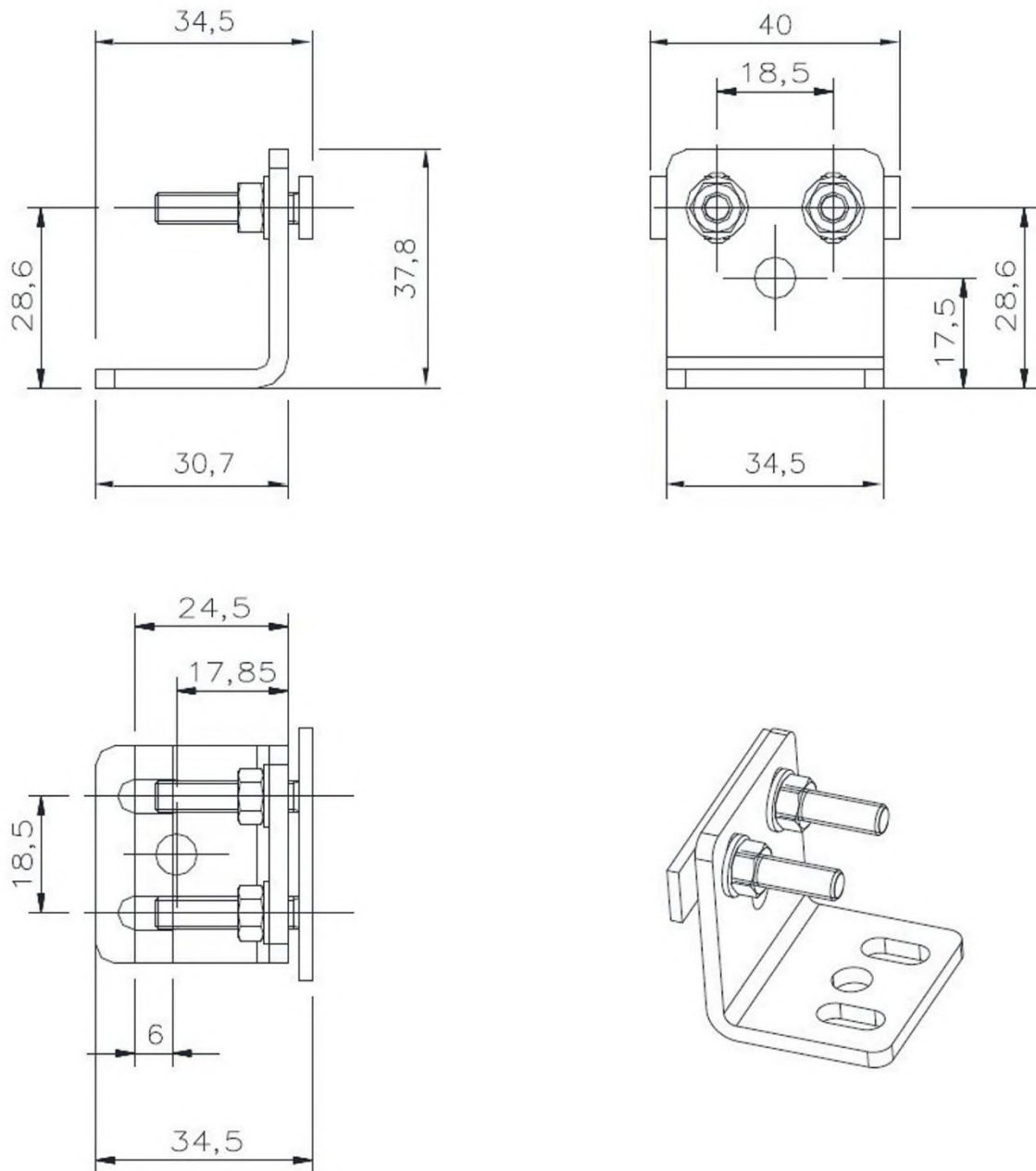
Fig 76 - Dimensions (mm)
