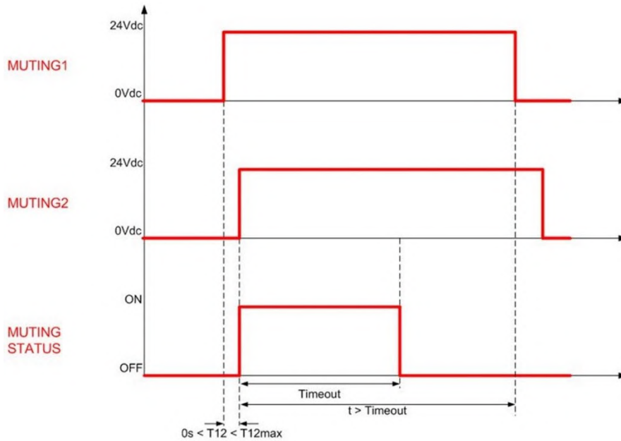
Fig 63 - Muting timeout
