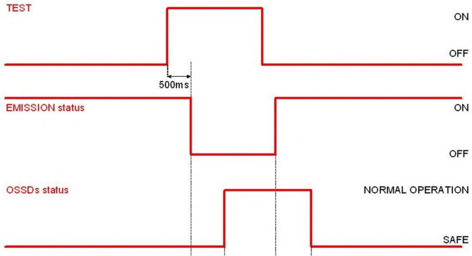
Fig 46 - Test timings
