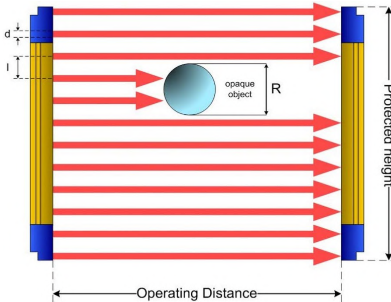
Fig 2 - Detection capability
