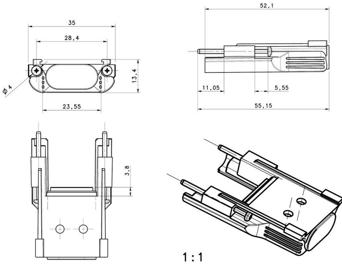
Fig 77 - Dimensions (mm)
