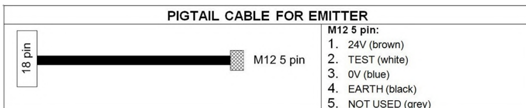
Fig 26 - Pigtail cable - configuration for emitter TX (CS-G1-50-B-002)
