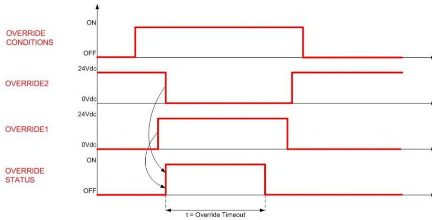
Fig 71 - Override timeout timings
