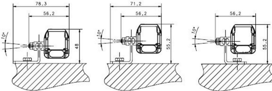
Fig 81 - Angled fixing bracket + Orientable support
