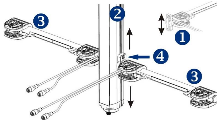
Fig 118 - Phase 1
