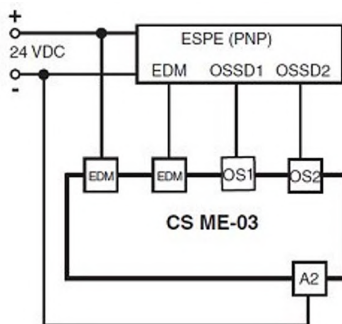
Fig 103 - EDM Relay
