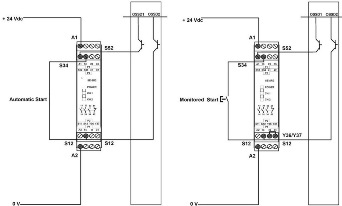
Fig 102 - Safety relay
