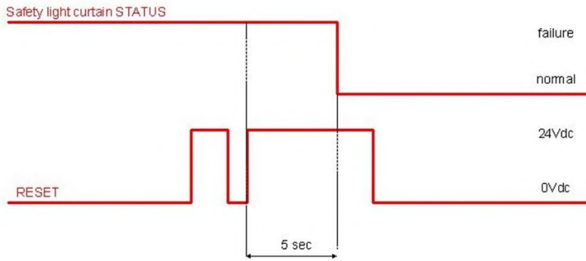
Fig 47 - Reset timings
