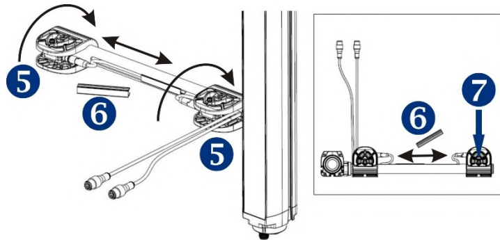
Fig 119 - Phase 2
