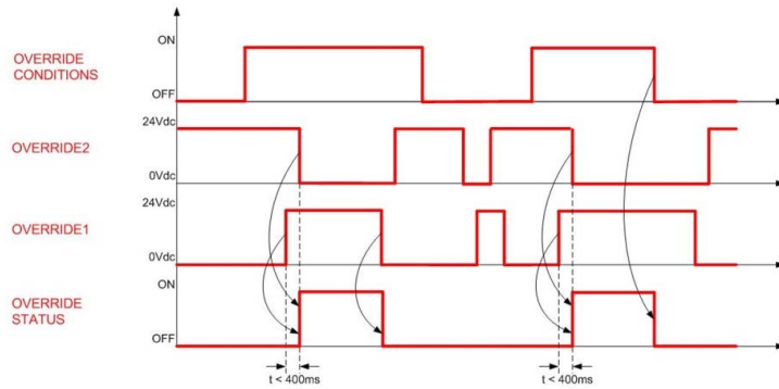
Fig 68 - Override timings (level trigger)
