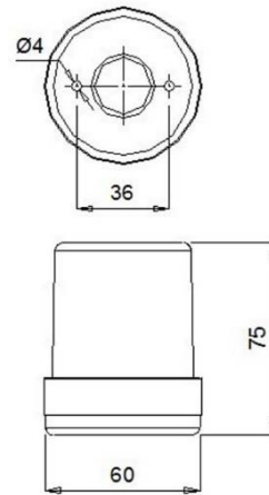
Fig 105 - Lamp LMS-2
