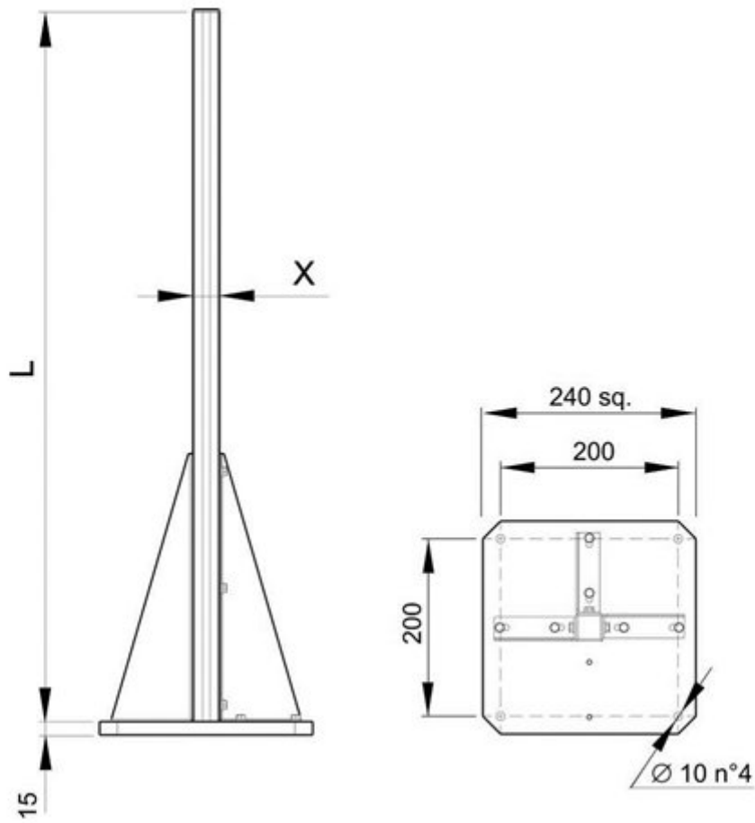
Fig 93 - Dimensions (mm)
