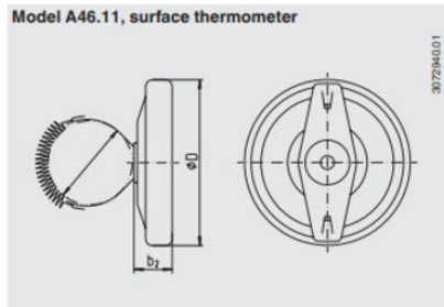
Model A46.11, surface thermometer
