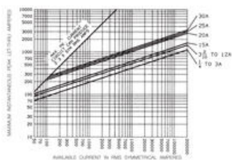
Peak Let-Thru Current Data - ATDR 1/4 Bll 30, 600 Volts AC
