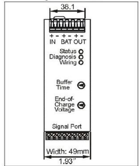
Fig. 24-2 Front view
