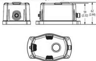
Figure 2 - Stainless Steel Housing (mm (in.))
