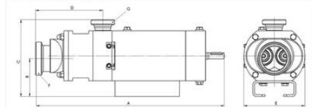
Mäz HYGHSPIN Extended H1 axel (mm)
