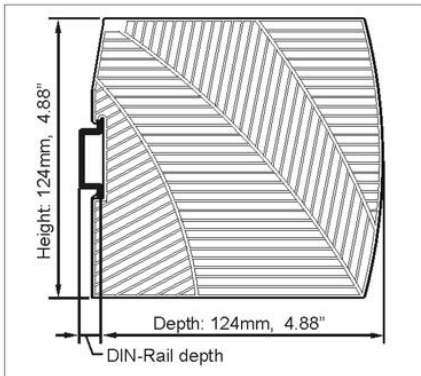
Fig. 20-3 Side view
