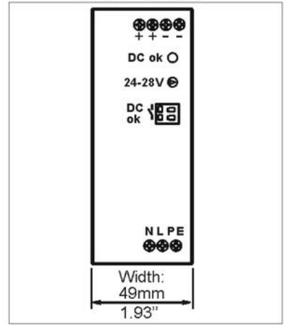
Fig. 20-1 Front view
