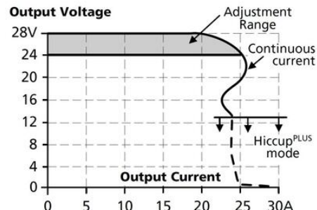
Output Voltage
