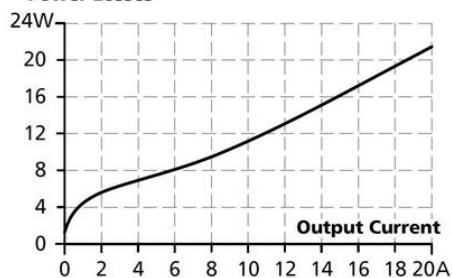
Power Losses
