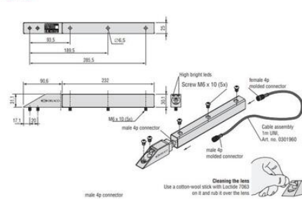
Front Side Molded Male connector
