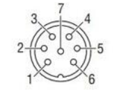
Front side molded 7P Male connector
