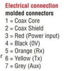
Front side molded 7P Female connector
