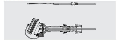
Fixed connection (compression fitting) to the furnace
