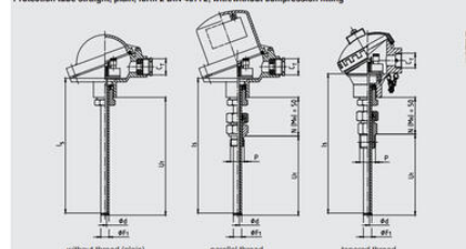
Protection tube straight, plain, form 2 DIN 43772, with/without compression fitting
