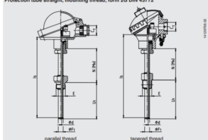
Protection tube straight, mounting thread, form 2G DIN 43772
