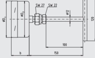
Model A73, with contact bulb Back mount (BM)
