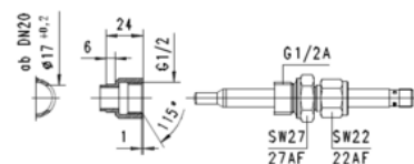
weld-on adapter
