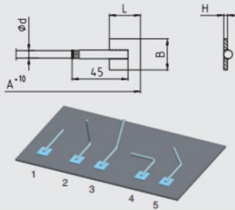
Weld-on sheet
