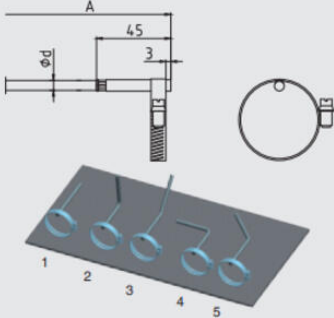
Tightening strap
