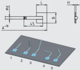
Weld-on sheet
