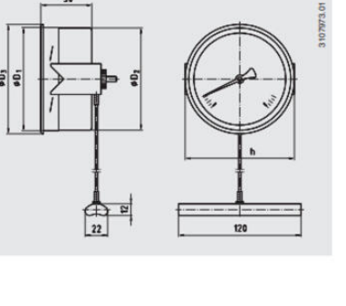
Model F73, with contact bulb Capillary and triangular bezel with clamp
