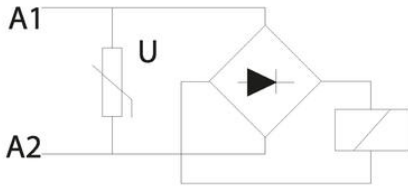
Coil circuit
